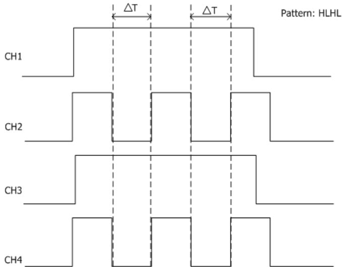
Figure 5-7 持続時間トリガ
